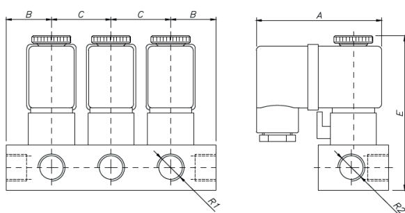
Bloco com bobina Mini**
